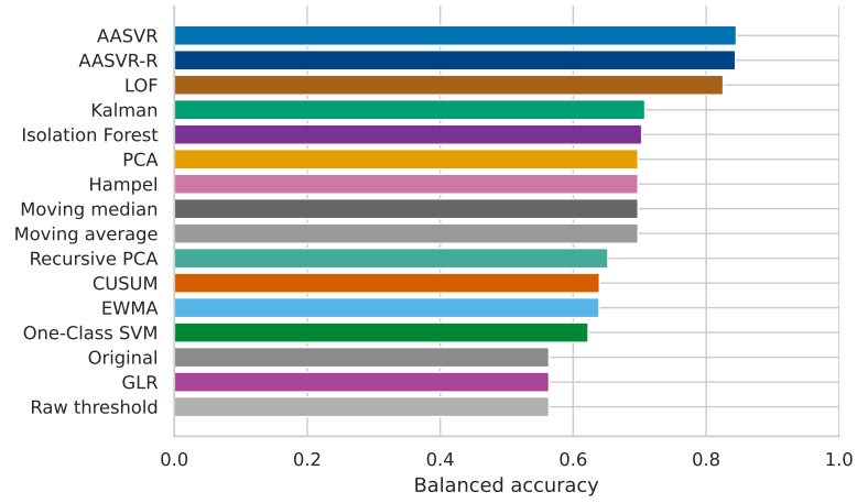
Figure 5: Held-out hydroponic synthetic-fault balanced accuracy across methods. AASVR-R combines robust gates with a CUSUM residual test and response-aware authorization, giving the strongest displayed balanced-accuracy/false-actuation tradeoff.
